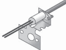
Completed assembly of Nitride replacement kit should look like this.
